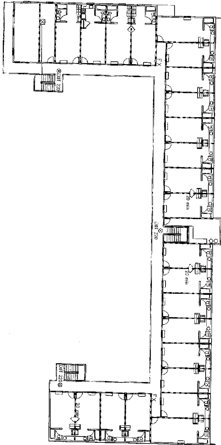
FOUNDATION PLAN 1 1/16" = 1'-0"
